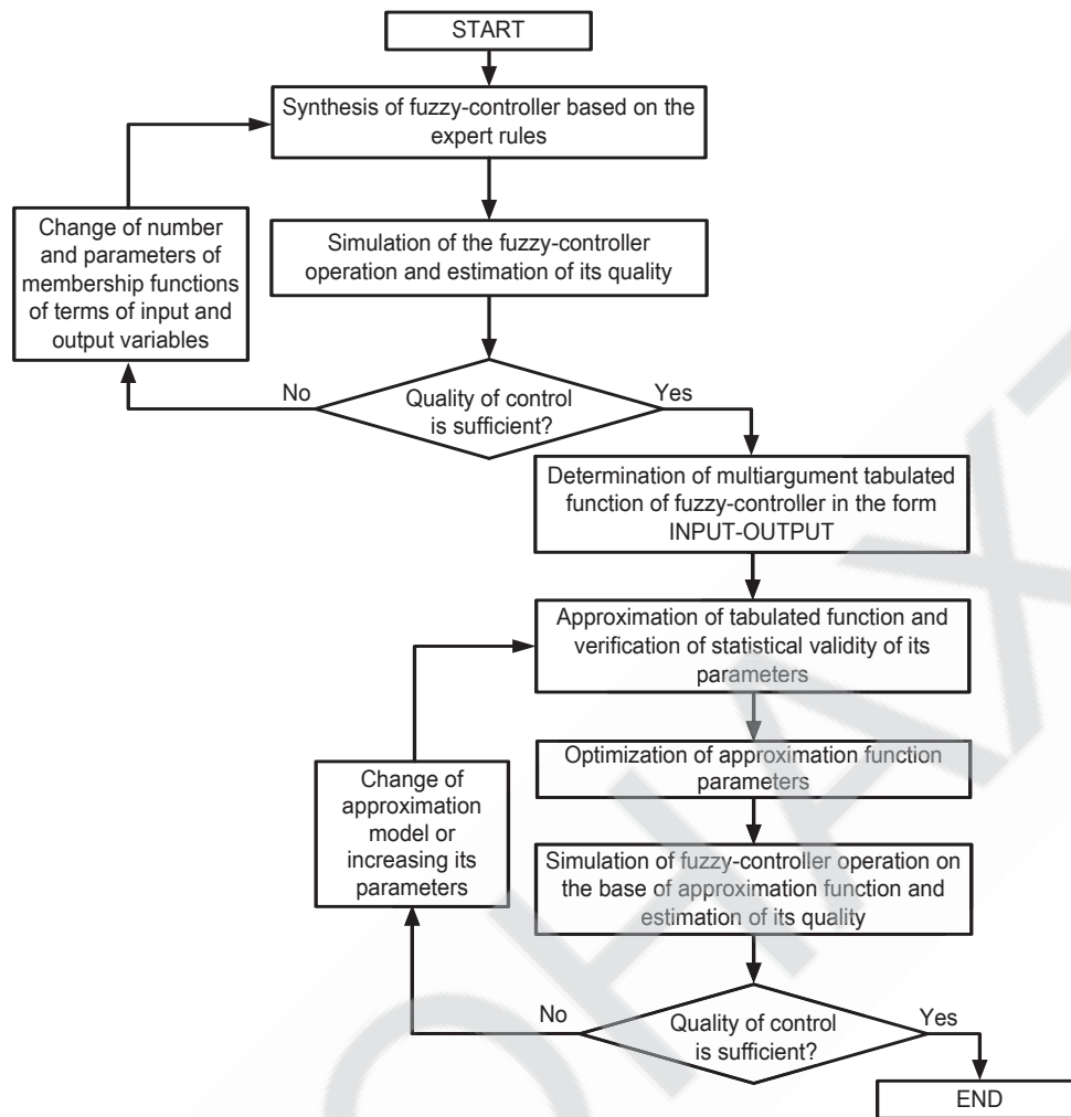
Fig. 1. Block-scheme of the method of synthesis of a fast fuzzy-controller
