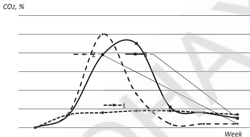
Fig. 4 - Change of CO_2 emissions from reactors during composting process of the composted mixture in reactors with microbiological additive in mesophilic (2) and thermophilic modes (3) in comparison with control sample (1), % CO_2
