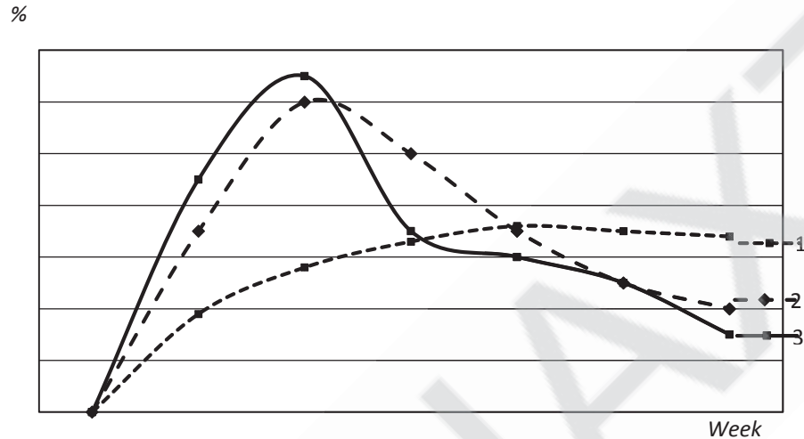
Fig. 5 - Change in the rate of loss of the total Carbon in a composted mixture in reactors with a microbiological additive in the mesophilic (2) and thermophilic modes (3) as compared to the control sample (1),% / week
