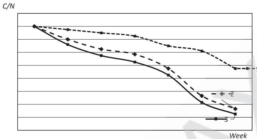
Fig. 9 - Changes in the ratio of total Carbon to total Nitrogen in a composted mixture in microbiological reactors in the mesophilic (2) and thermophilic regimes (3) as compared to the control sample, g / kg per week
