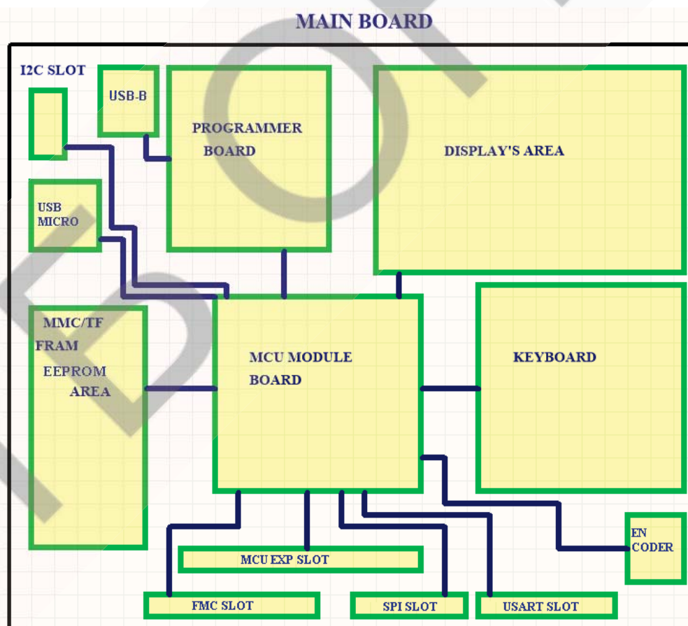
Fig. 1. Block diagram of the training kit
