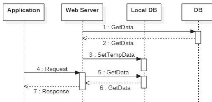
Figure 2 – Architecture with a local database
