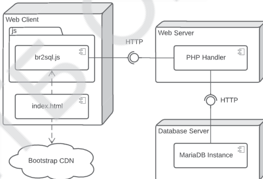
Figure 3 – Experimental stage software architecture
