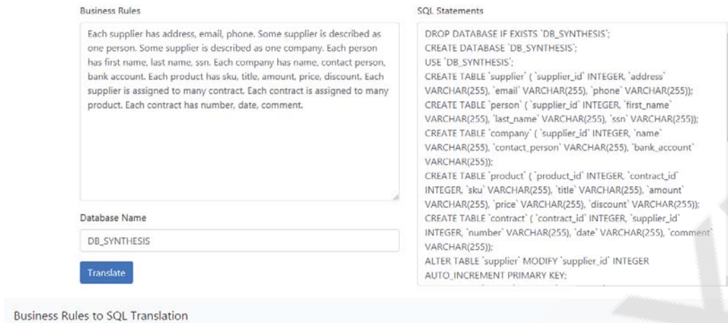
Figure 4 – User interface of the developed software prototype
