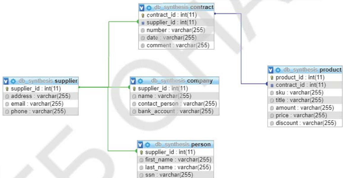
Figure 5 – Deployed database structure
