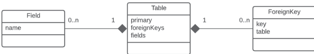
Figure 1 – Parsed business rules metamodel
