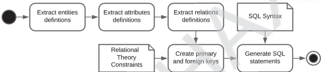
Figure 2 – Business rules into SQL statements translation sequence
