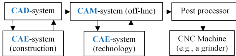
Fig. 1 Integrated system CAD/CAM/CAE in mechanical engineering technology
