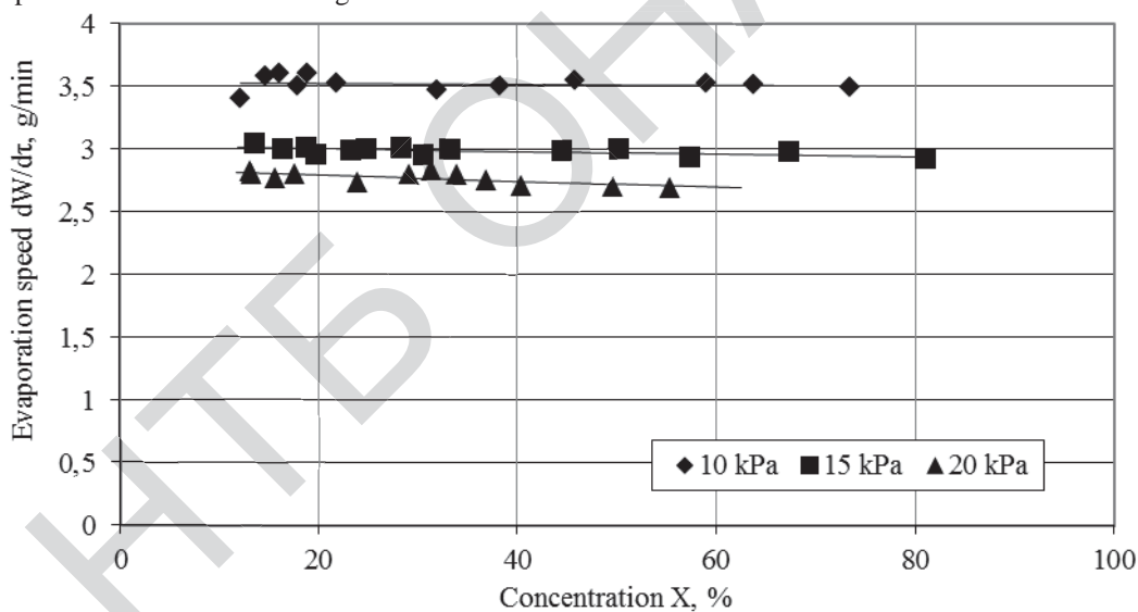
Figure 4. The pressure effect on the apple juice evaporation speed
