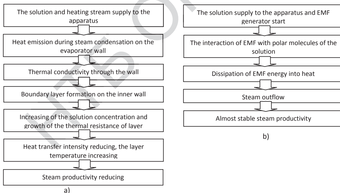
Figure 1. Thermophysical model of evaporation processes: a) – traditional technology; b) – innovative technology
