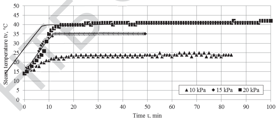
Figure 2. The pressure effect on the temperature of the apple juice evaporation process
