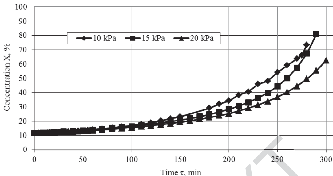
Figure 3. The pressure effect on the kinetics of changes in the apple juice concentration
