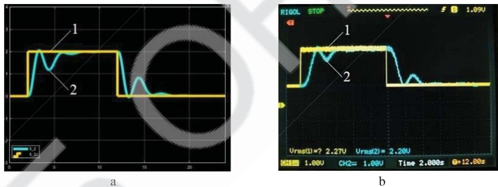
Figure 3. The charts of the signal of the second mass position \varphi_2 and the position assignment \varphi_{2a} : a - mathematical model, b - physical model.
