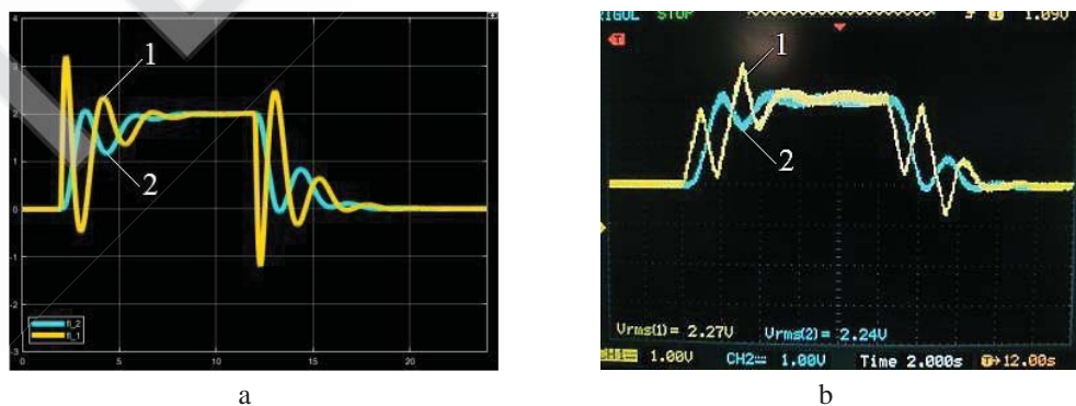
Figure 4. The charts of the transients of the position of the first \varphi_1 and the second \varphi_2 mass: a - mathematical model, b - physical model.
