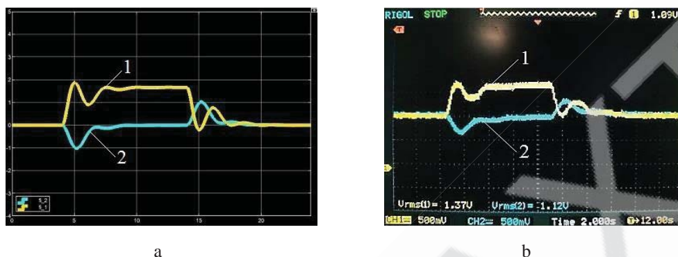
Figure 5. Graphs of the transients of the position of the first \varphi_1 and second \varphi_2 masses with the motor running and when applying M_r : a - mathematical model, b - physical model.
