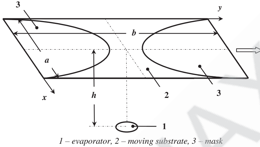
Fig. 1 Schematic diagram showing continuous thin film deposition with a mask.
