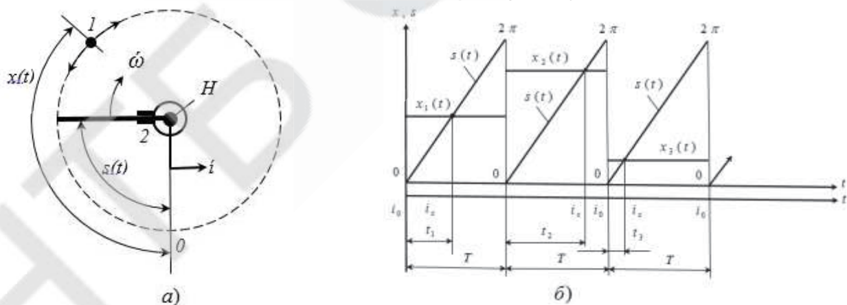
Fig.2. Geometric scanning system
