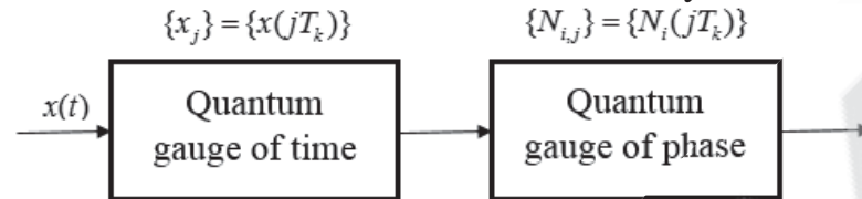
Fig.1. Functional scheme of ADC
