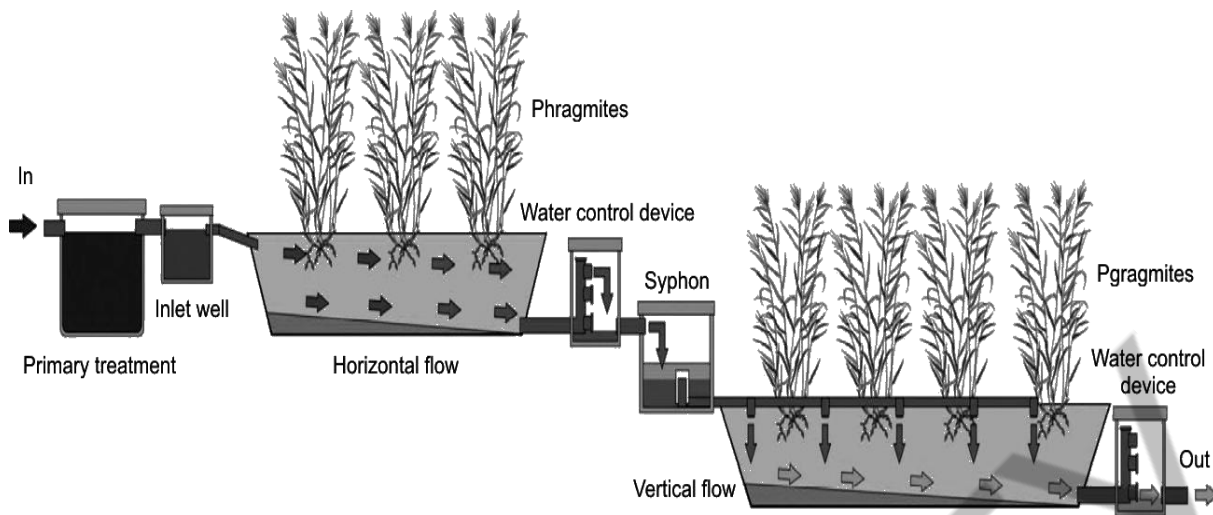
Fig.2. Scheme of hybrid constructed wetlands with HF and VF beds
