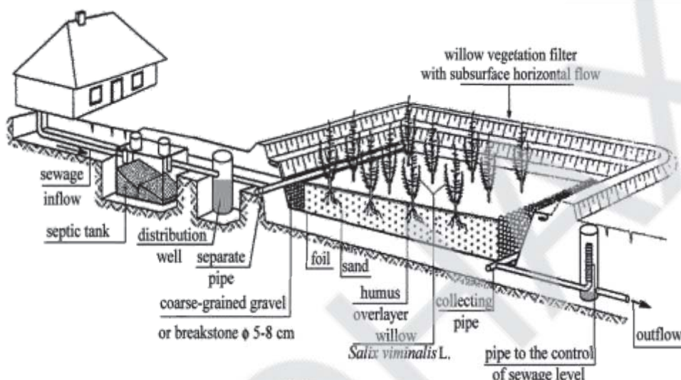
Technological scheme of one stage constructed wetland with subsurface horizontal flow [Drupka et al. 1992]
