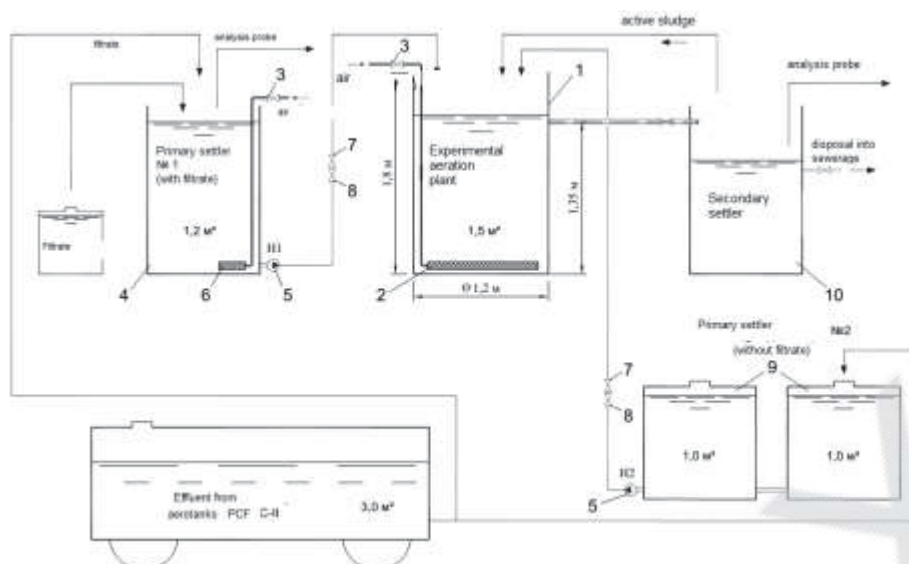
Experimental plant for tertiary infiltrate treatment
