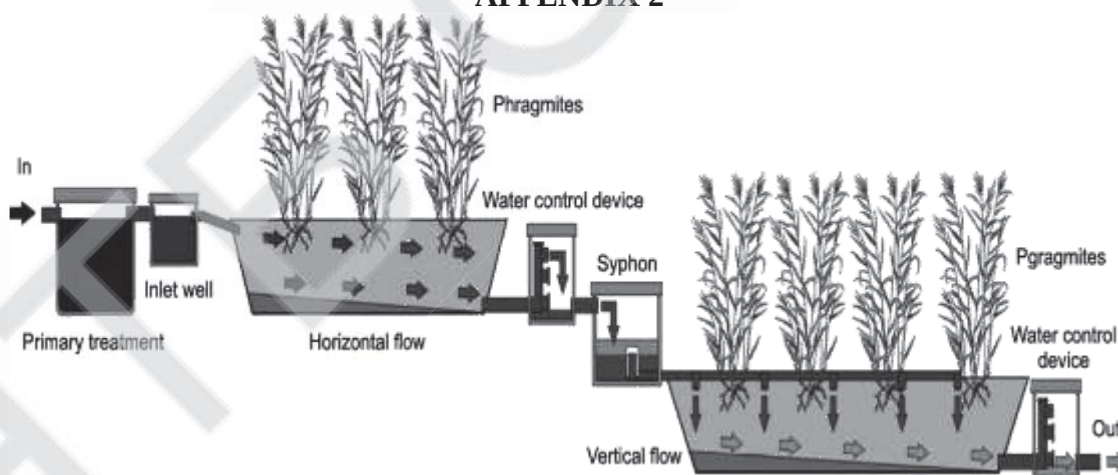
Scheme of hybrid constructed wetlands with HF and VF beds [Masi, Martinuzzi 2007]
