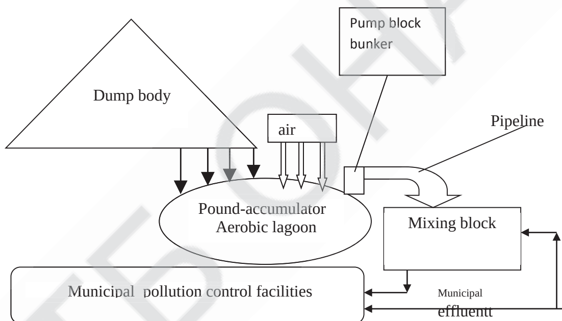
Principal scheme of two-stage landfill infiltrate purification in aerobic lagoons and at municipal pollution control facilities
