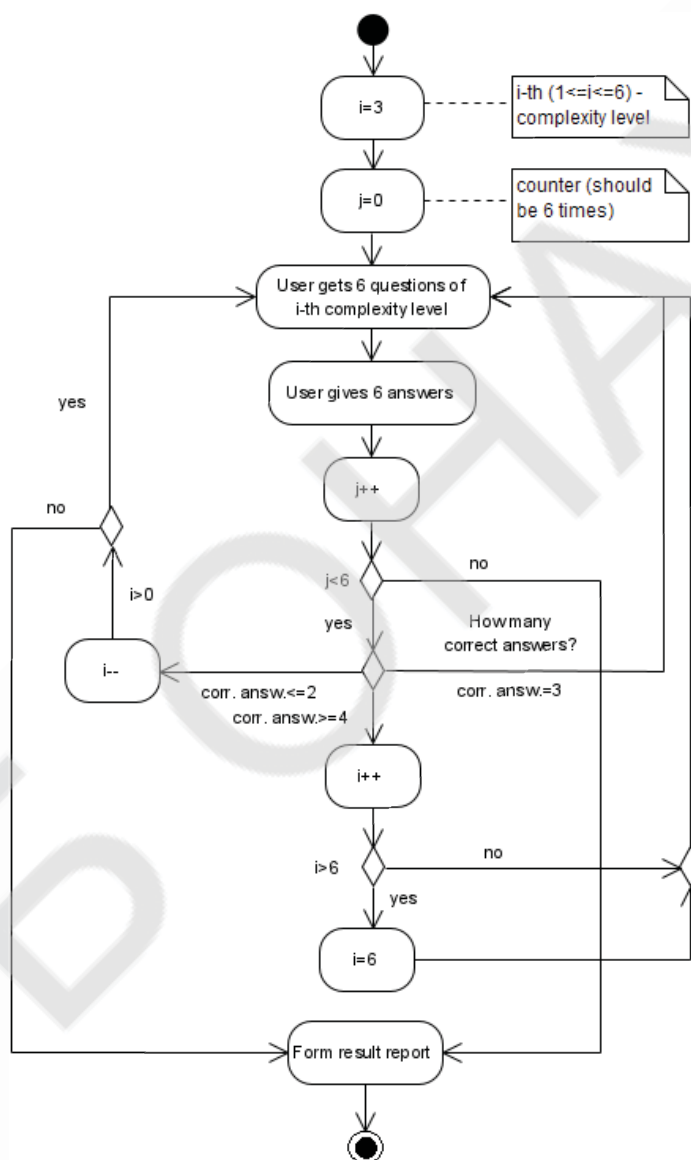
Figure 2 – Adaptive testing algorithm
