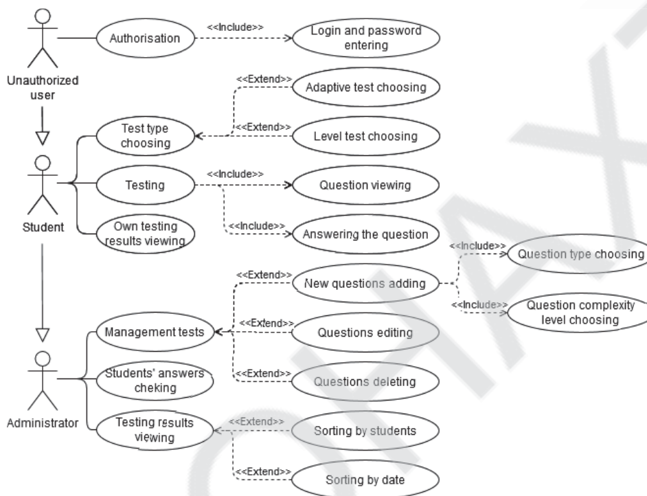
Figure 1 – Use-case diagram
