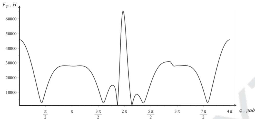
Fig. 1. The effect of the specific load on the connecting rod neck of the crankshaft of the internal combustion engine.
