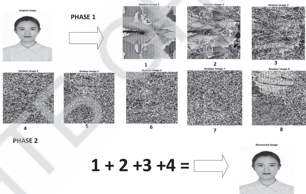
Fig. 1. An example of experimental sharing / restoration of a secret in the form of a graphic image according to Shamir's scheme (4,8): (a - the original image, b - secret shares (subsecrets), c - image reconstructed in 4 shares, Phase 1 - secret separation, Phase 2 - recovery secret). Quality indicators of the reconstructed image: CC = 0.945 , Q = 301.6 .
