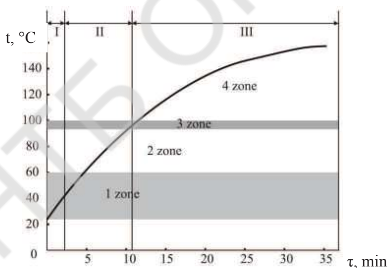
Fig. 1 – Temperature characteristics of periods and zones of the bread baking process
