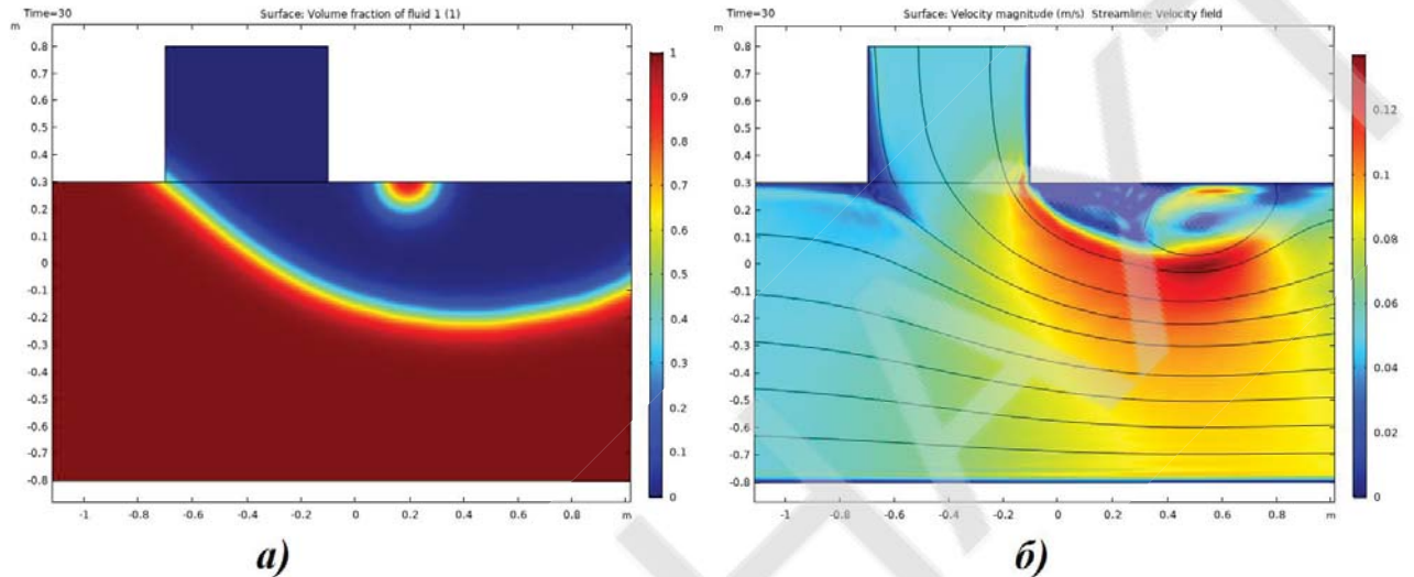
Figure 1. Two-phase flow of the "liquid-liquid" type, realized using the Level set interface a) volume fraction function distribution b) velocity magnitude diagram and streamlines
