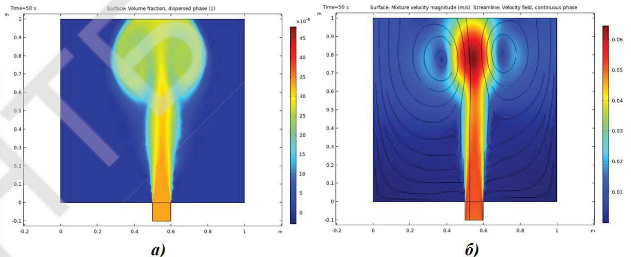
Figure 2. Two-phase flow of the "liquid-liquid" type, realized using the Euler-Euler model a) volume fraction function distribution b) velocity magnitude diagram and streamlines
