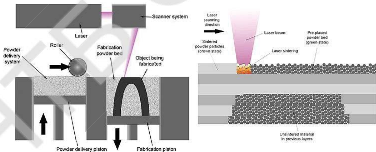
Fig. 2 - SLS printing technology
