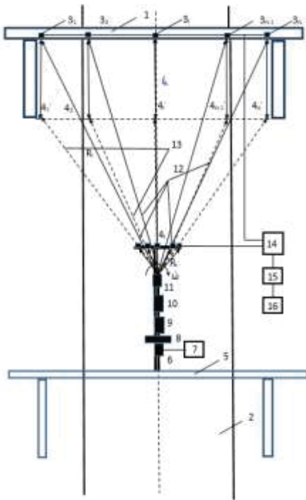
Picture 6. General appearance of the device without deformation of the bridge bulkhead
