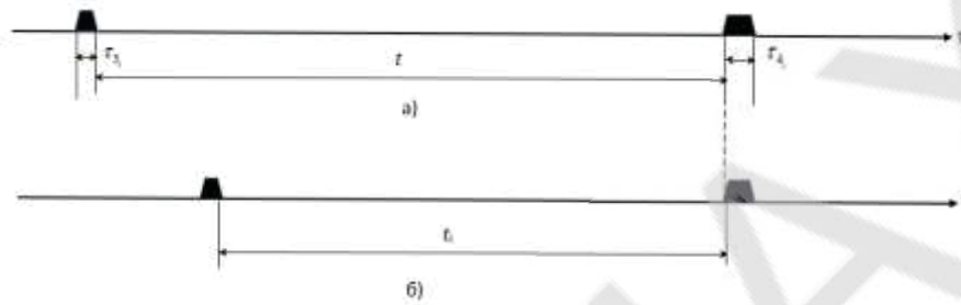
Picture 8. Time diagrams of operation of the device without deformation of the bridge span (a) and after deformation (b).
